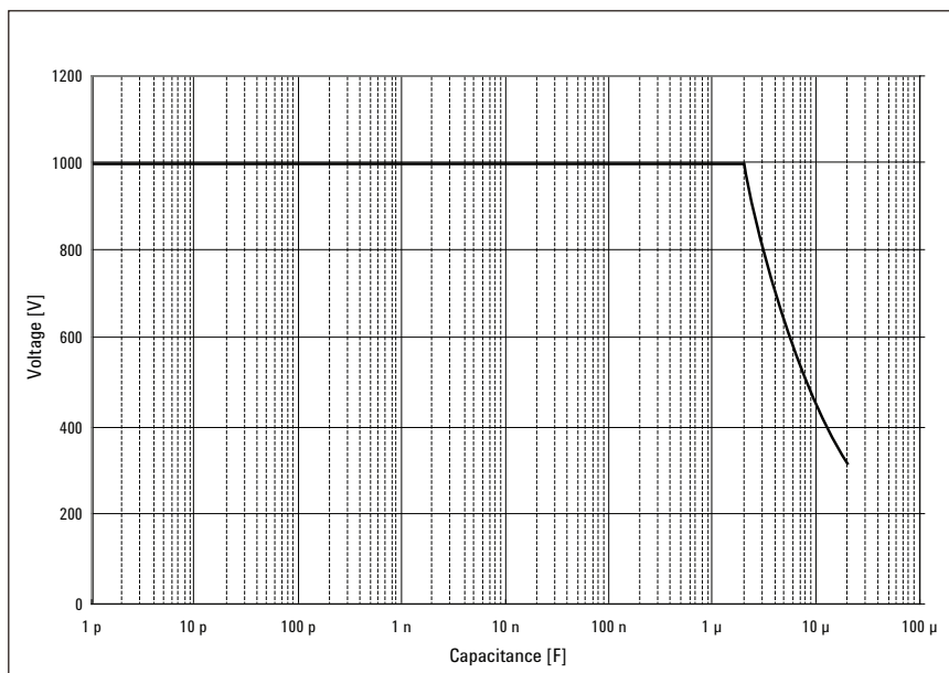
Figure 13. Maximum discharge withstand voltage (typical)
